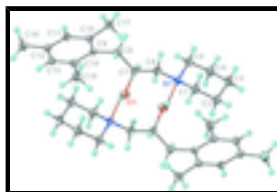
Fig. 1. Anisotropic displacement ellipsoid plot (Barbour, 2001) of the hydrogen-bonded dimeric structure of C 17 H 27 NO at the 70% probability level; hydrogen atoms are drawn as spheres of arbitrary radius.
